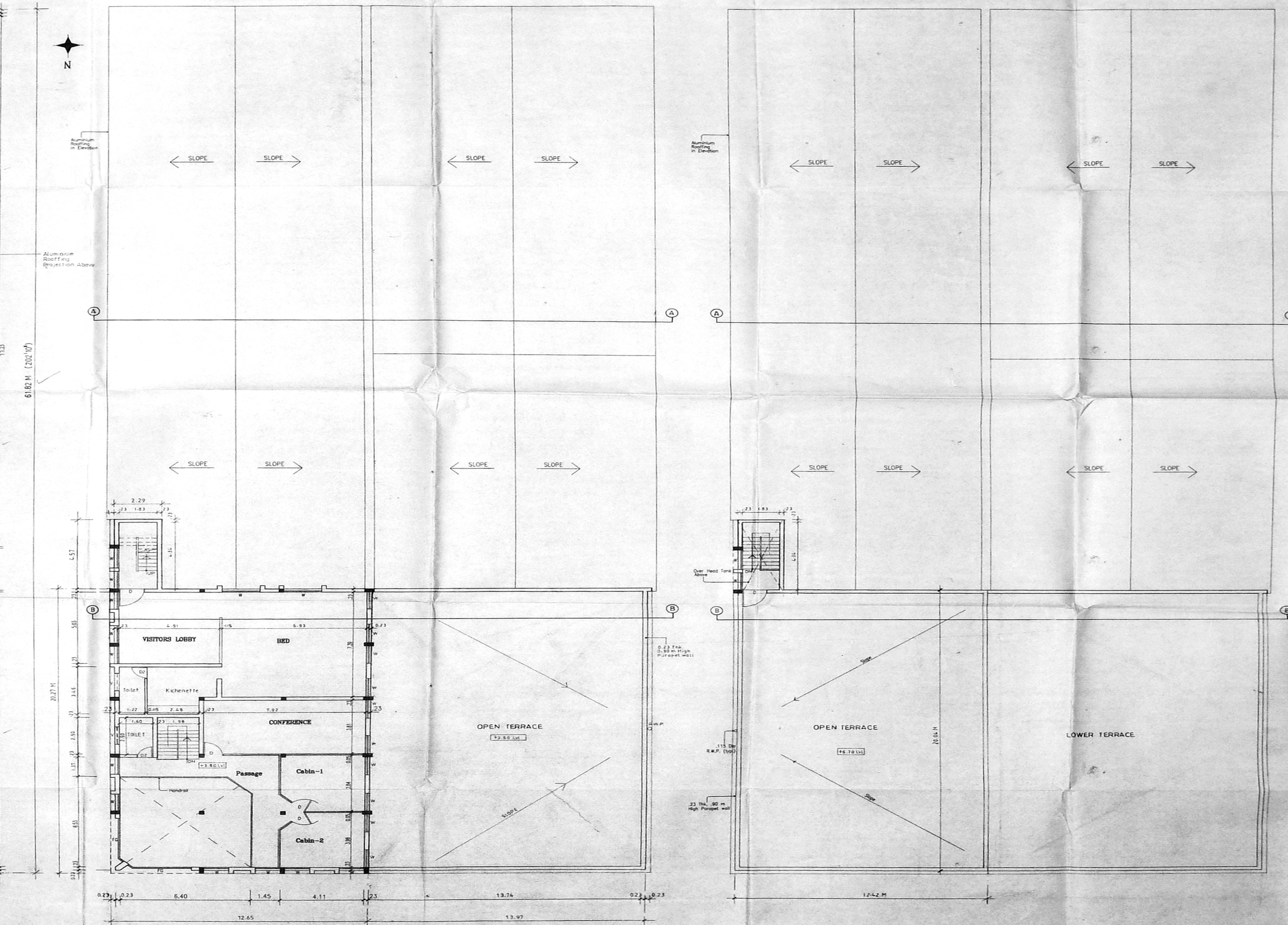
TERRACE PLAN
